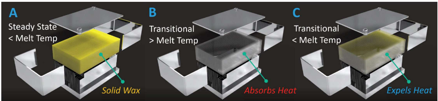
Figure 2: Exploded View of Sealed PCM Heat Sink Through Phase
